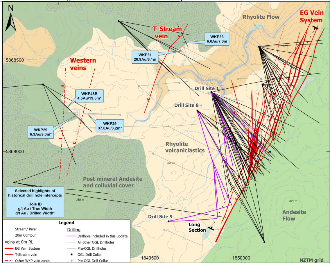
Figure 1: WKP plan view of geology, drill traces, and distribution of 3 main vein zones. Note: T- Stream and Western Vein intercepts are significant historical results (full results are provided at https://investors.oceanagold.com/additional-drillhole-data ).
